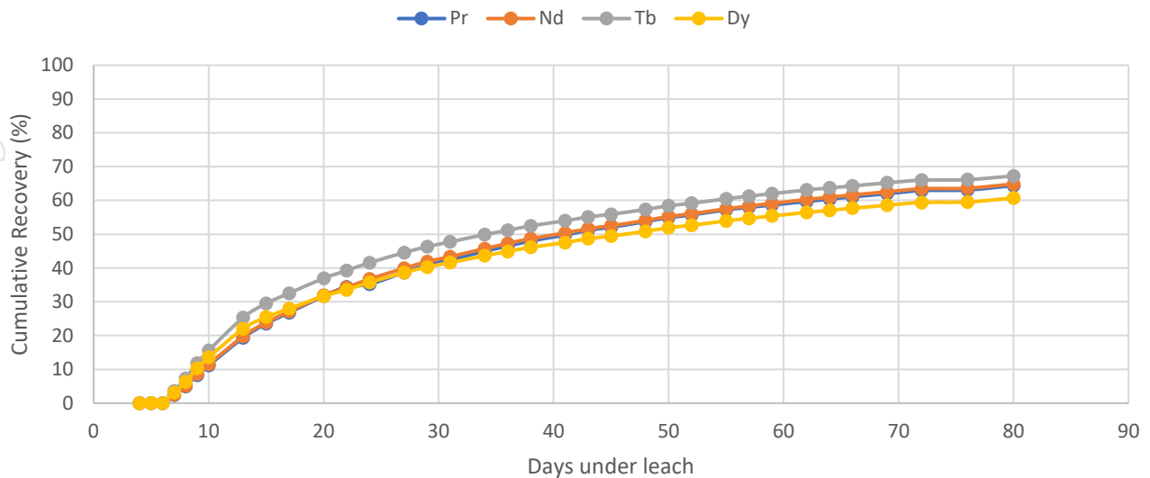
Figure 3: Prop Composite Heap Leaching Results – Cumulative Recovery by Day
