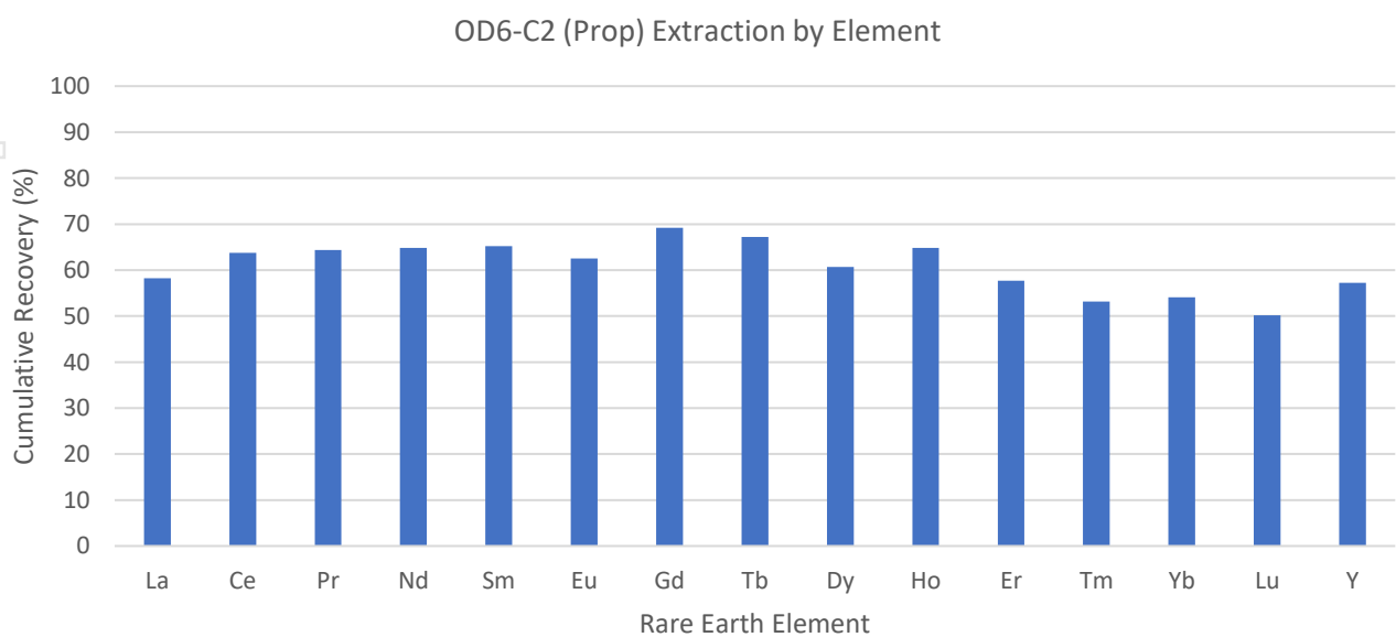
Figure 4: Prop Prospect Column Leach REE Recovery by Element
