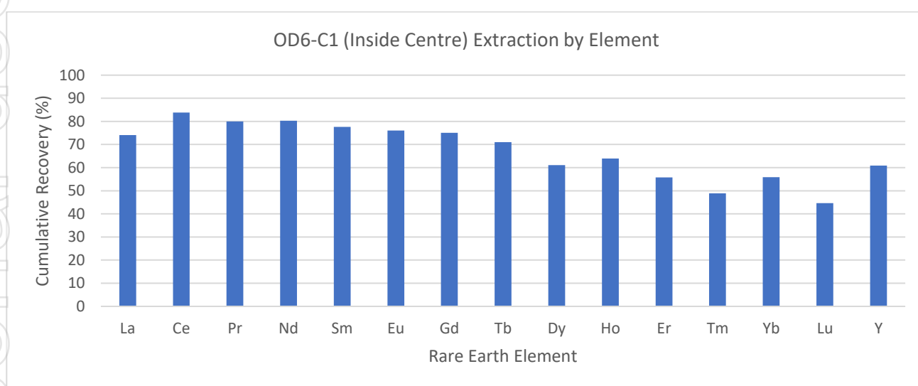
Figure 2: Inside Centre Column Leach REE Recovery by Element
