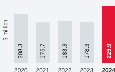
Cash
