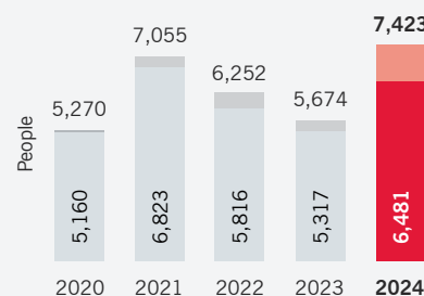
Workforce numbers
