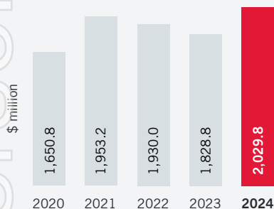
Revenue 1
