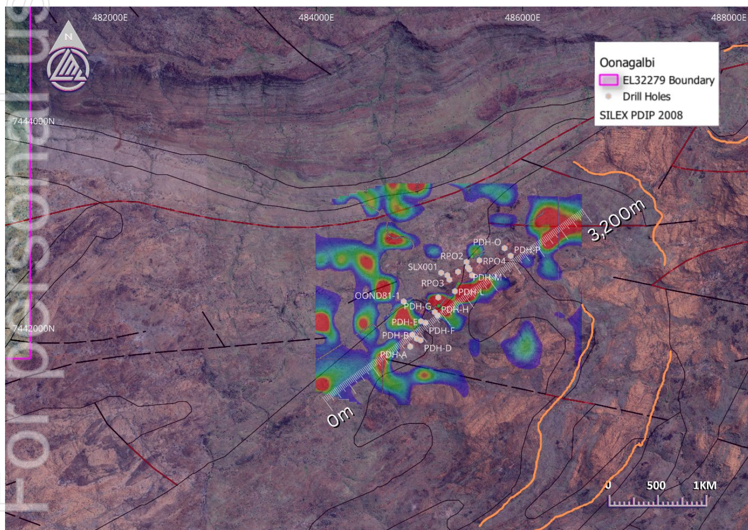
Figure 3. Location of historic drill holes overlayed with the 2008 PDIP survey conducted with Silex. Orange zones are also highlighted as potential mineralised zones further IP should be conducted over.
