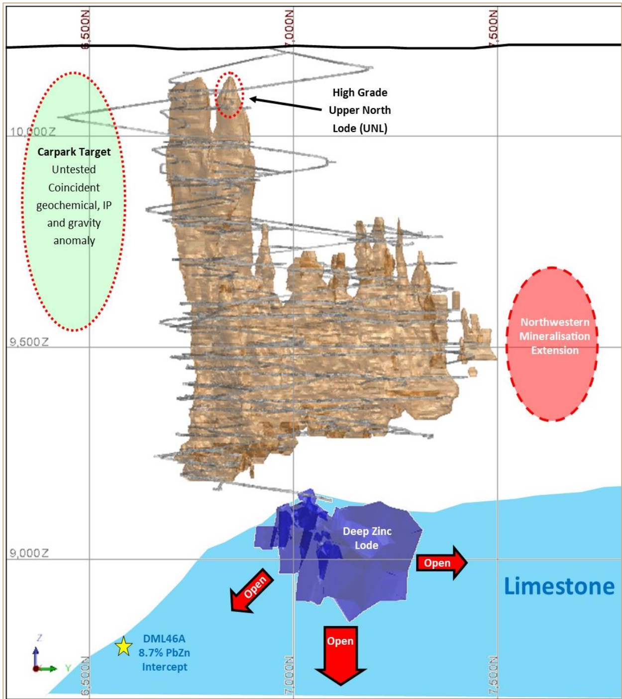
Figure 1. Section of the Endeavor Mine showing location of the high grade Upper North Lode (UNL)
