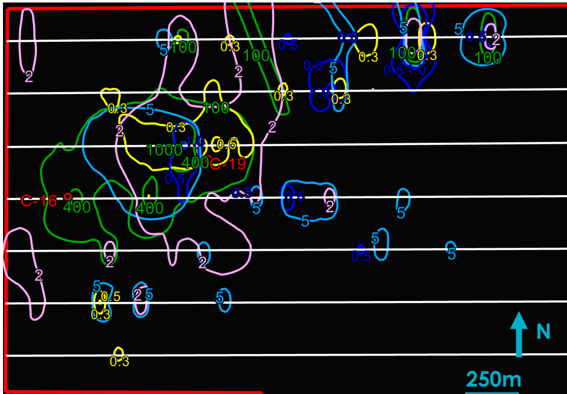
Figure 5 - Soil Anomalism at Ilken (ppm). White horizontal lines are sampling fences, 250m apart. Green Cu, Purple Mo, Pink Bi, Light Blue Sb, Dark Blue Ag (g/t), Yellow Te.
