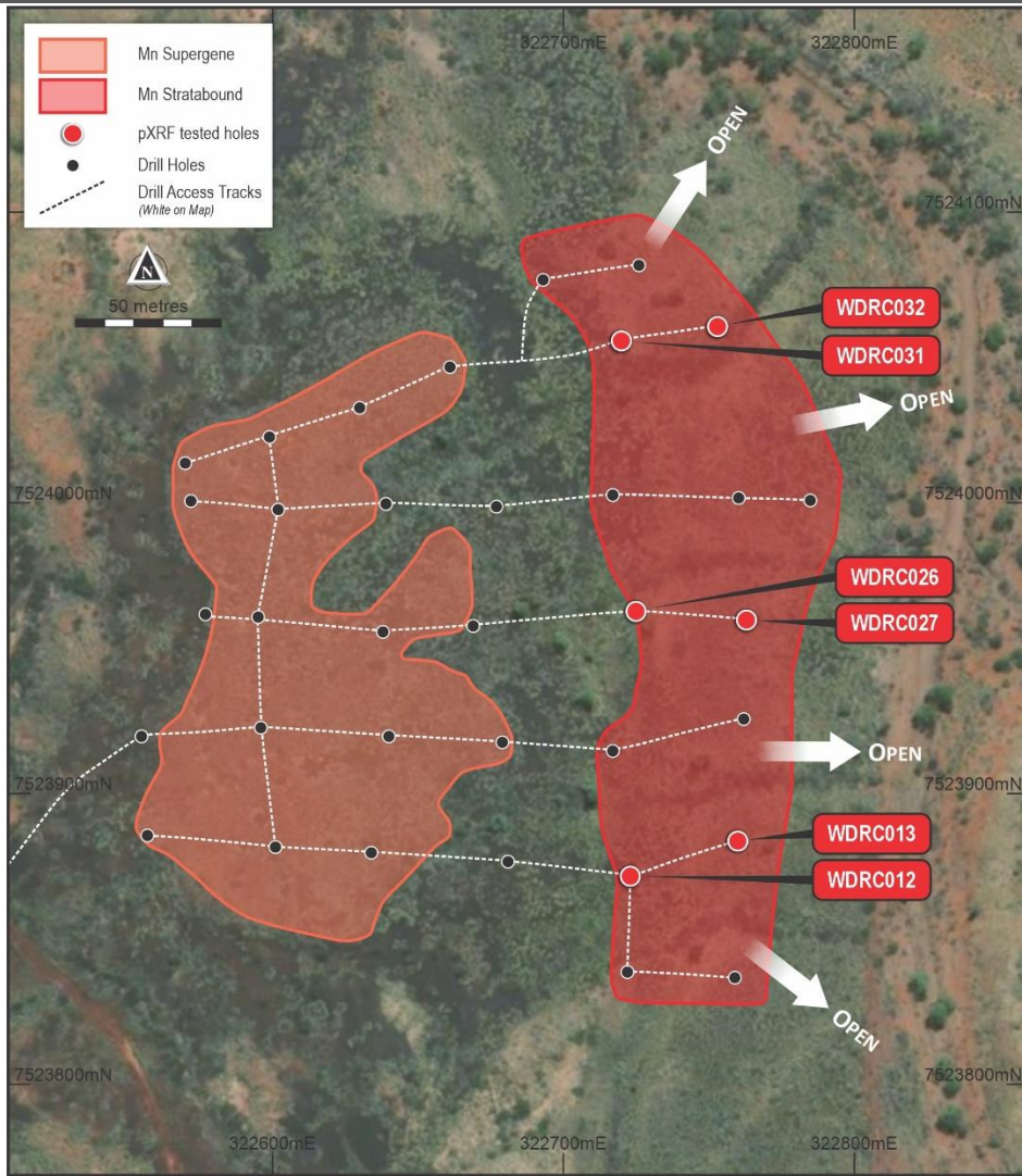
Figure 3. Drill collar location plan and stratabound mineralisation projected to surface.
