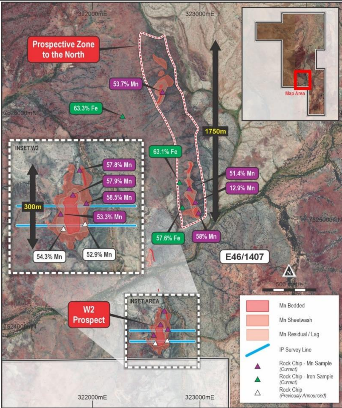
Figure 2. W2 prospect, Wandanya Project (E46/1407) showing high grade manganese outcrops and the IP survey lines
