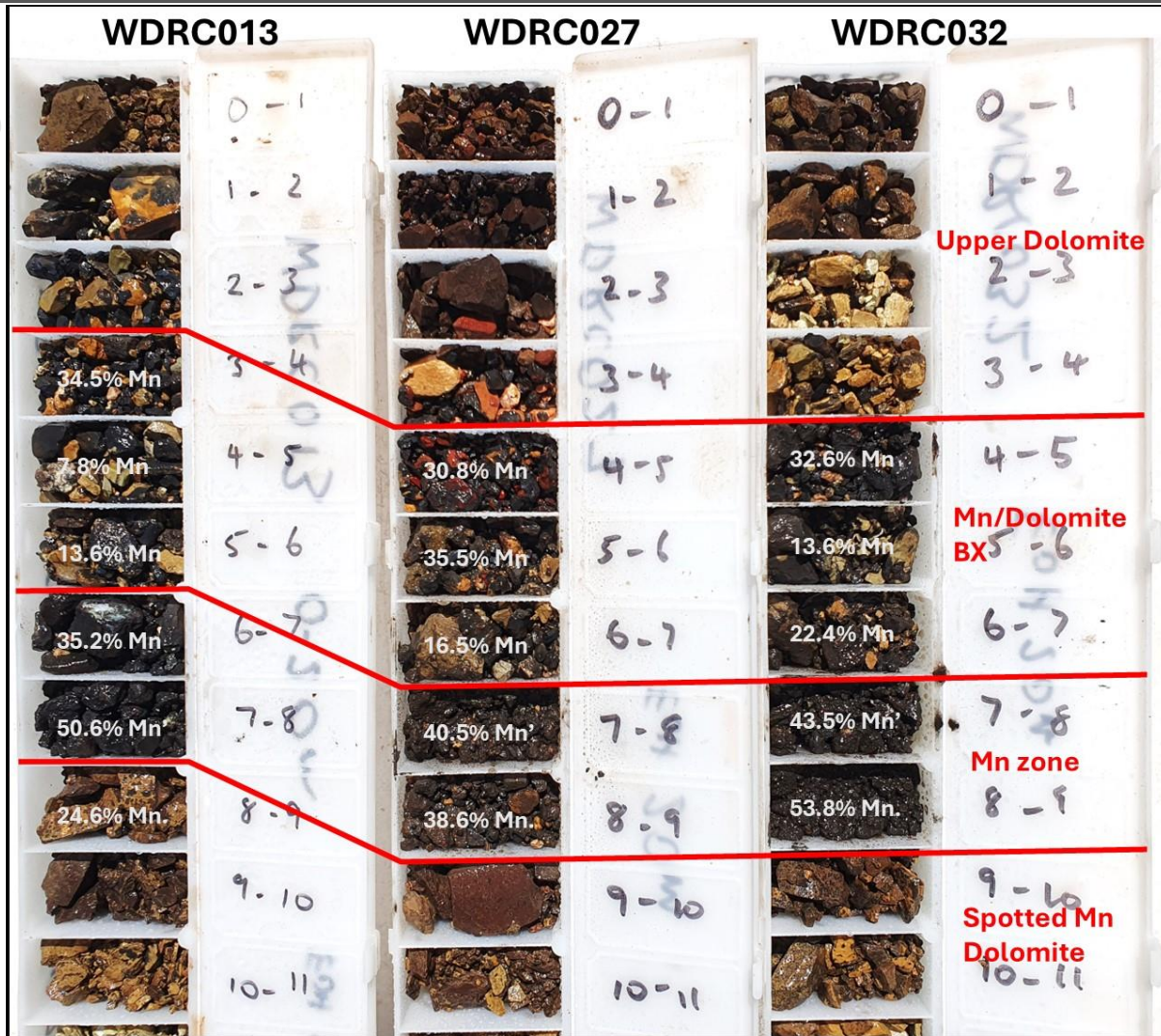
Figure 4. Chip tray photos from 0-11m from selected holes drilled into the W2 Prospect showing laboratory based assay result and various zones defined within the manganese horizon.
