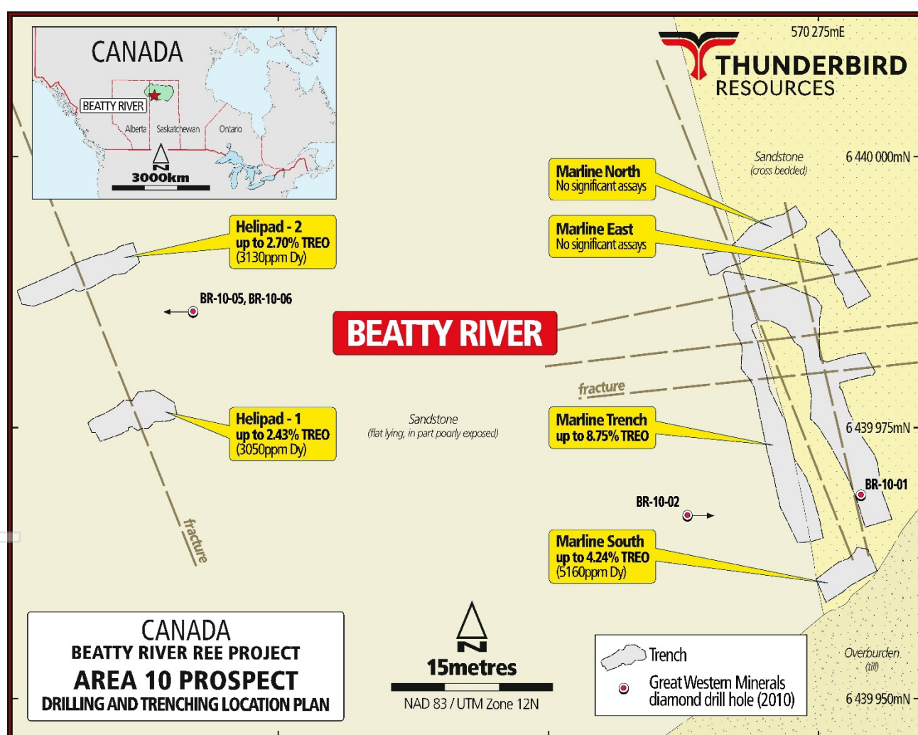
Figure 5: Beatty River Project – Historical Area 10 prospect showing historical drilling and surface sampling (highest TREO values labelled)
