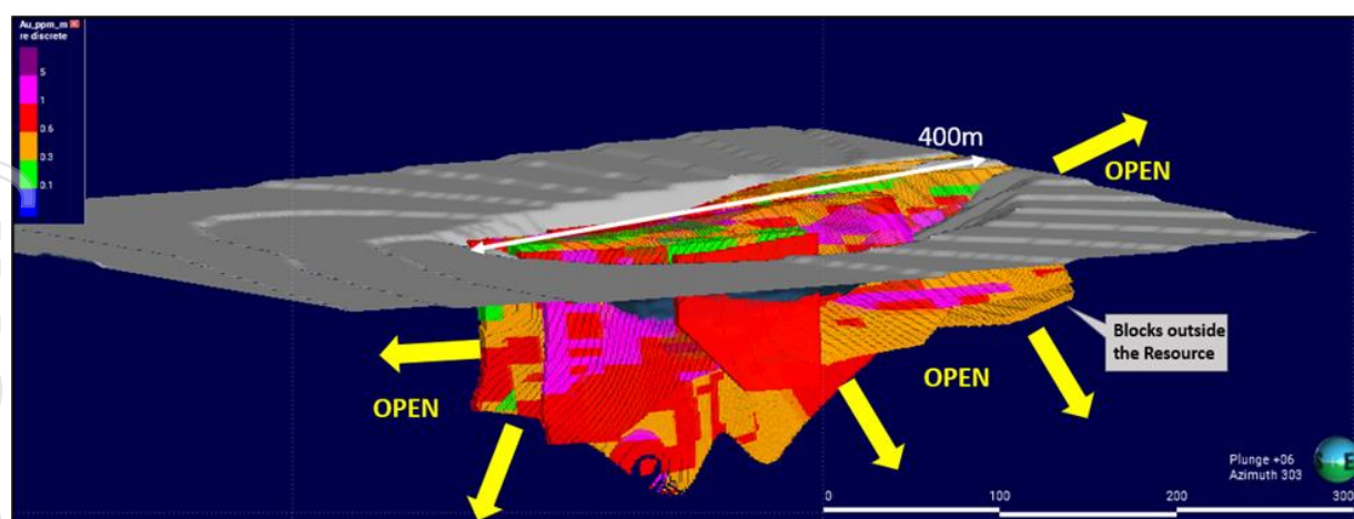
Figure 7: Berekko Mineral Resource 3D perspective view
