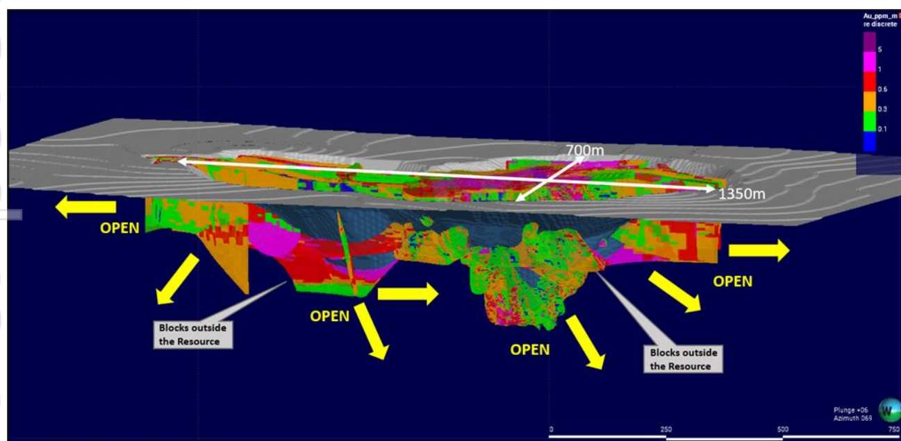
Figure 6: Massan Mineral Resource 3D perspective view, looking northeast
