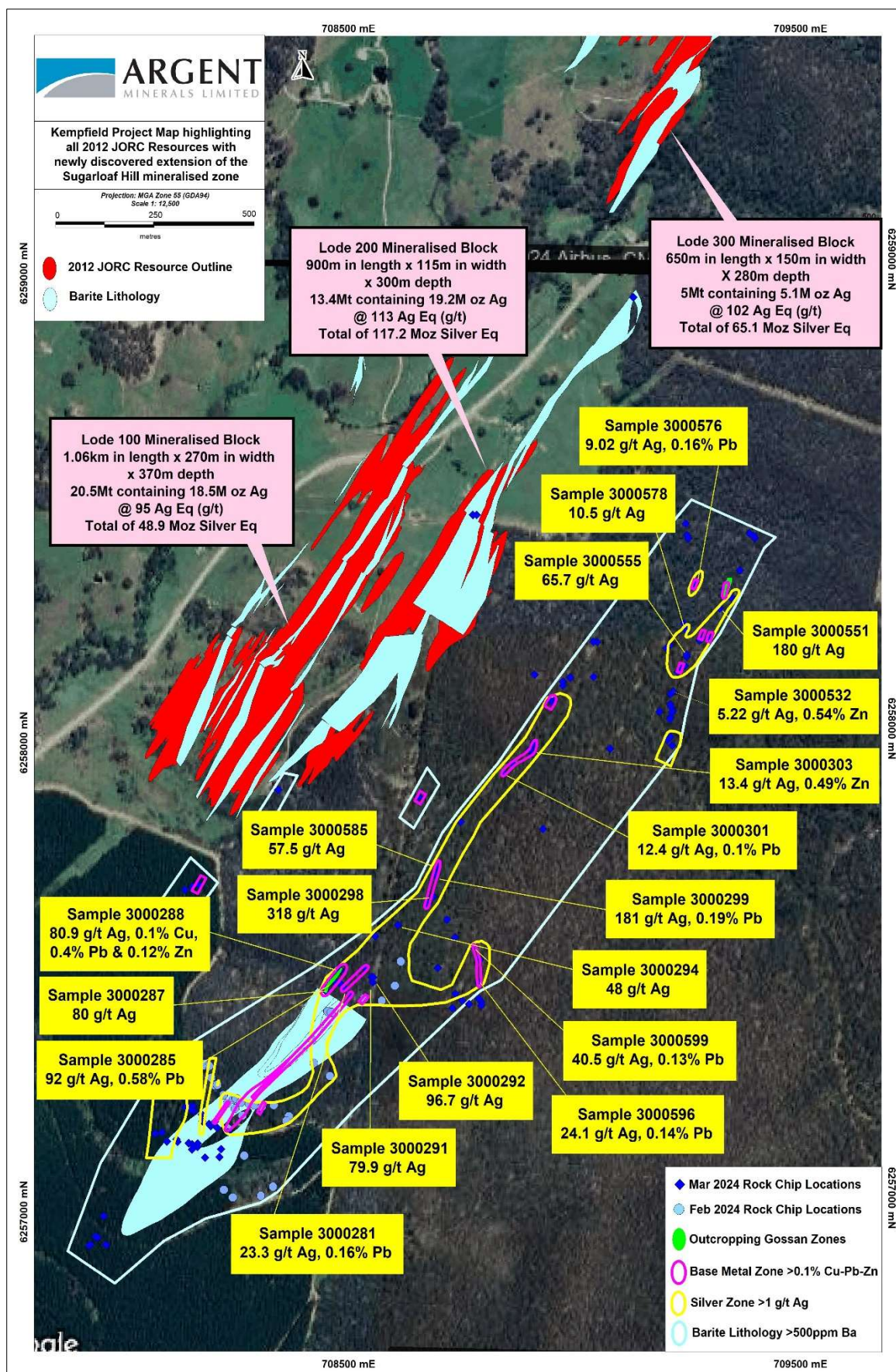
Figure 12 – Kempfield Project Location Map highlighting some of the high-grade rock chip results over the Sugarloaf Hill Zone
