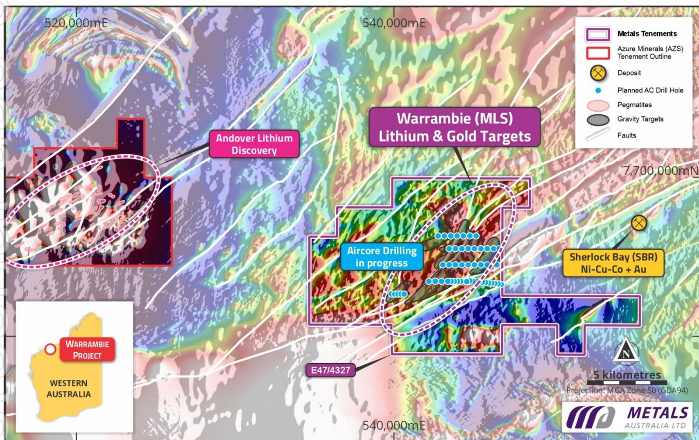
Figure 2: Warrambie Project E47/4327 reprocessed magnetics image, targets and nearby Andover lithium discovery
