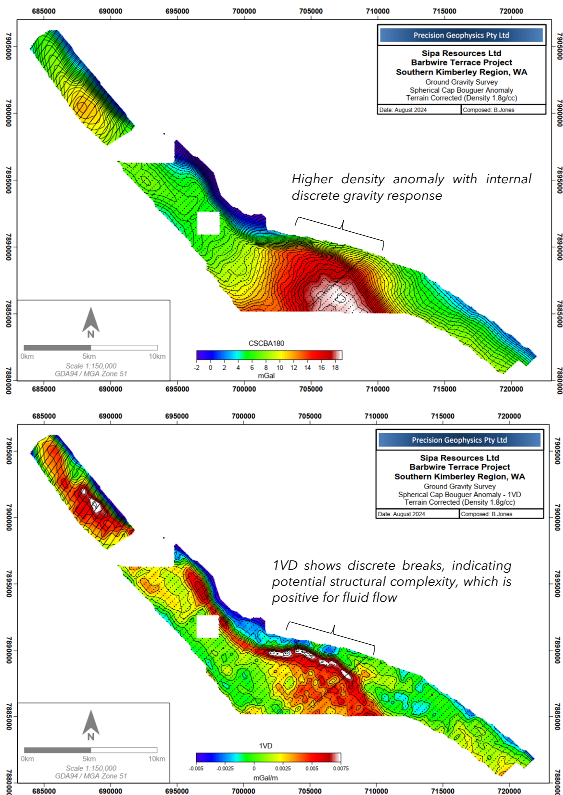
Barbwire Terrace Project: Detailed gravity survey data - Bouguer Anomaly (top) and Bouguer Anomaly 1 st Vertical Derivative (Bottom)
