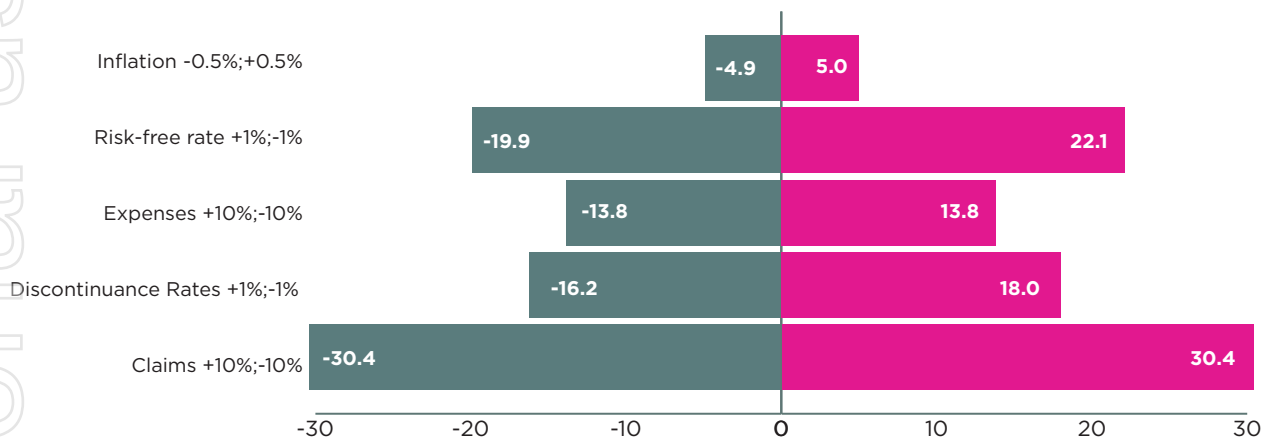
Chart 9: Embedded Value sensitivity analysis @ 4%DM
