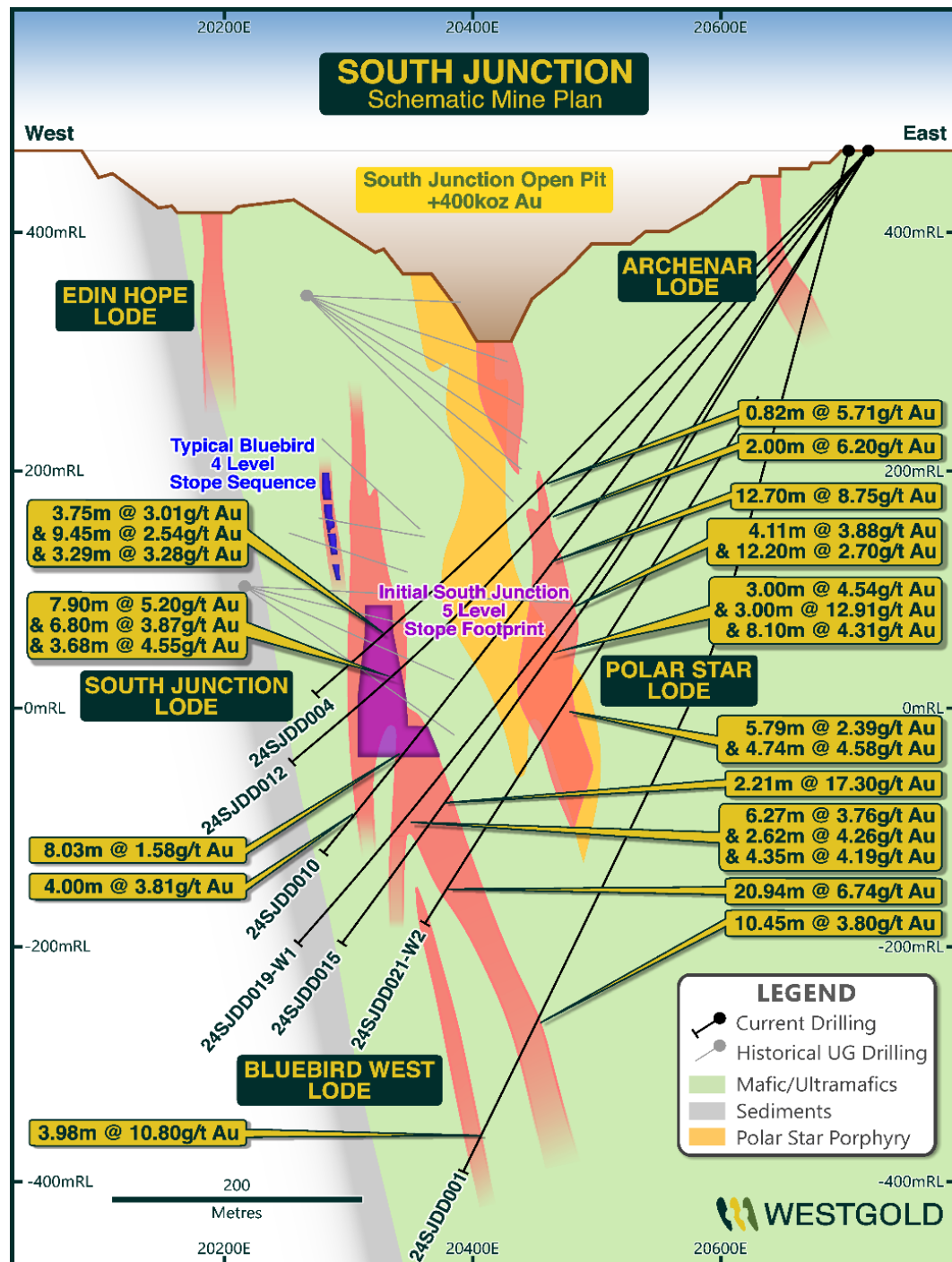
Figure 4 – South Junction schematic mine layout showing the scale of a typical South Junction stoping panel as compared to a typical stoping panel of the current Bluebird mine (Refer Appendix B for detailed drill results)
