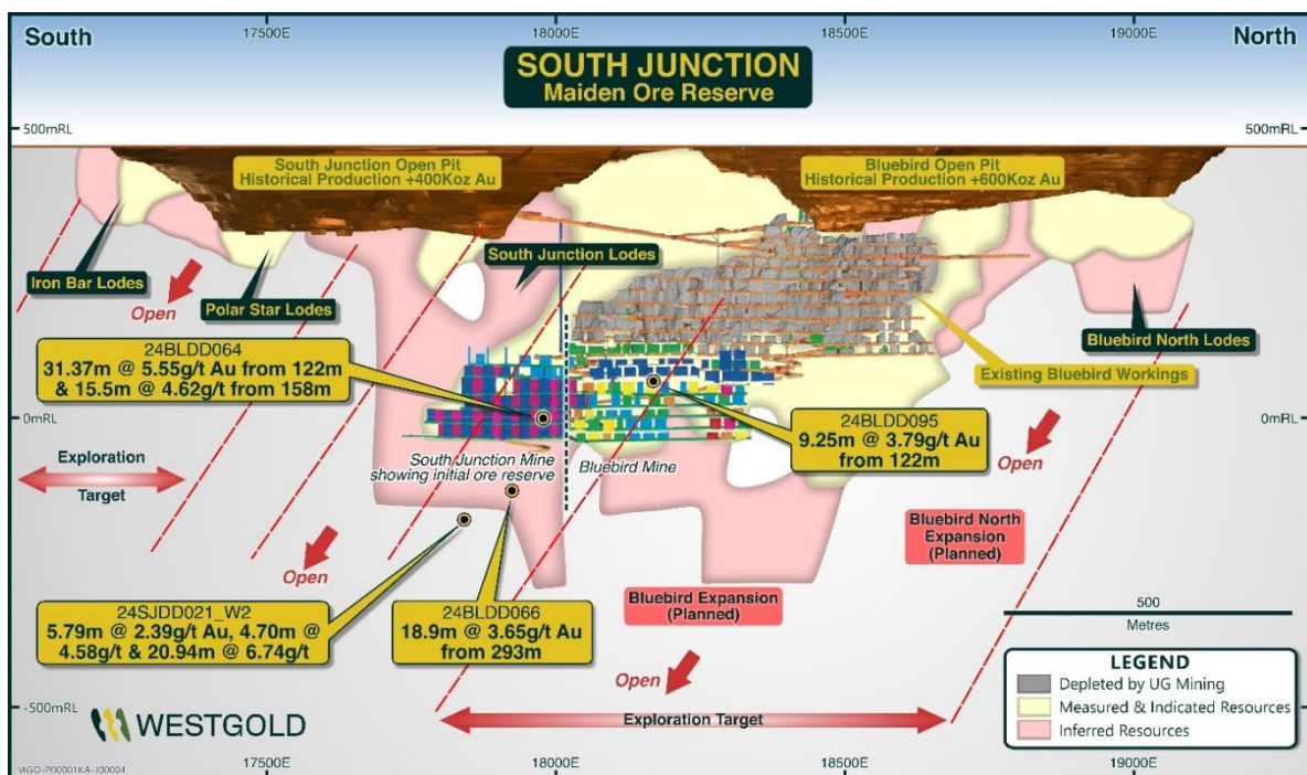
Figure 1 - Bluebird – South Junction underground complex showing footprint of current Ore Reserve
