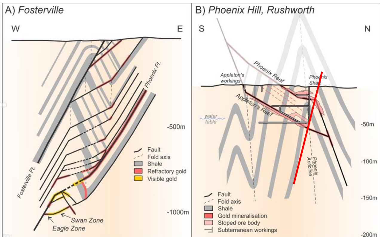
Figure 1: Phoenix Hill cross-section compiled from geological mapping completed by Jones & Turnbull (2014) and Boucher (2016). Figure modified from Dart Mining ASX November 2020. Planned drilling location shown in Red.
