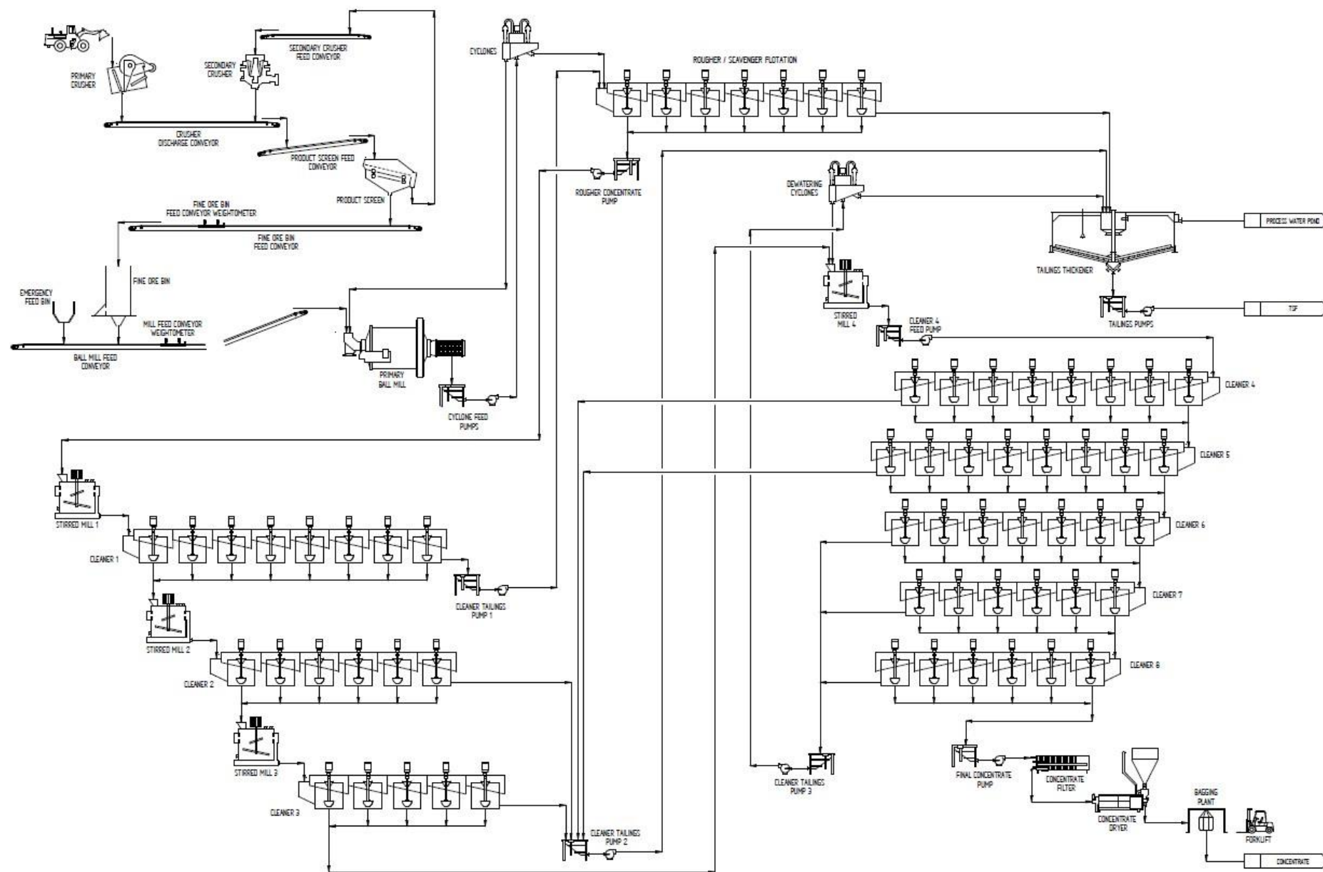
Figure 13 - Beneficiation Plant Flowsheet
