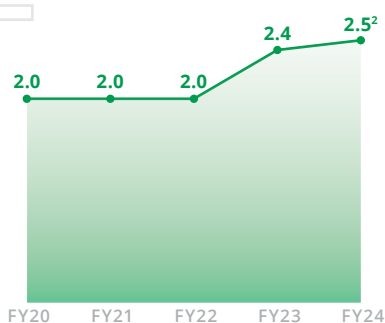
Figure 14: Average daily traffic (millions)
