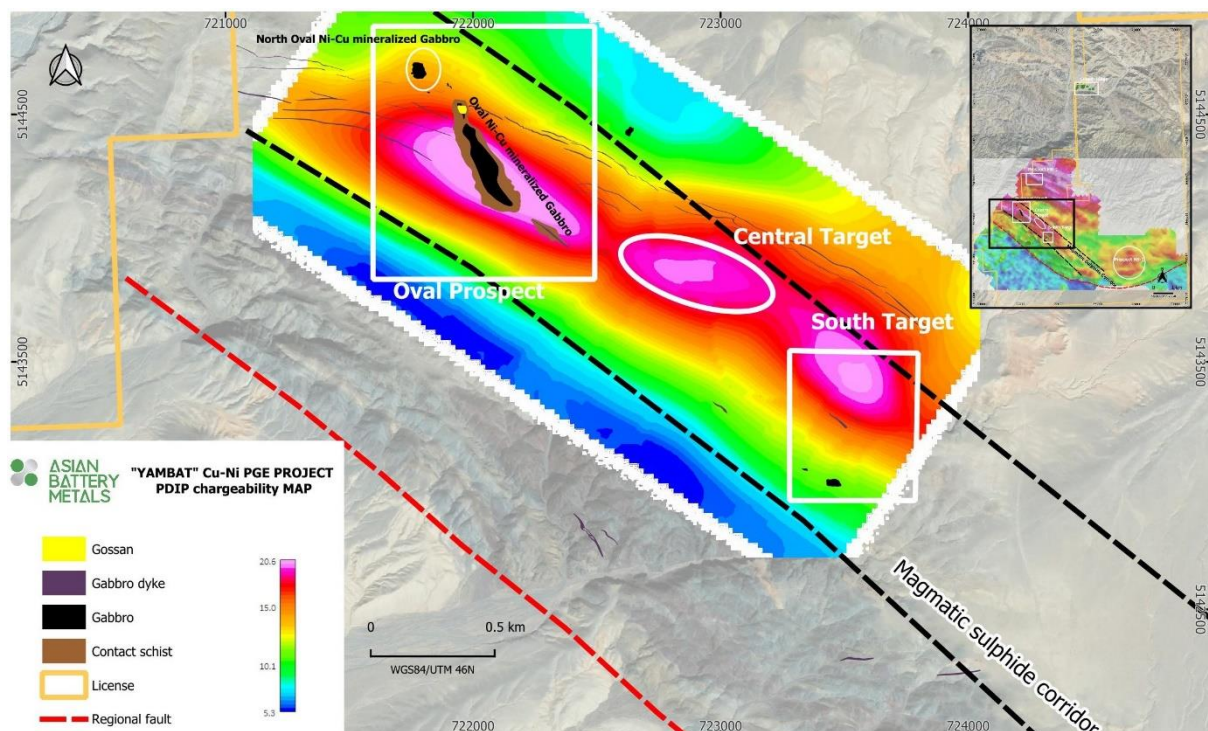
Figure-5. Spatial distribution of PDIP-defined chargeability anomalies.
