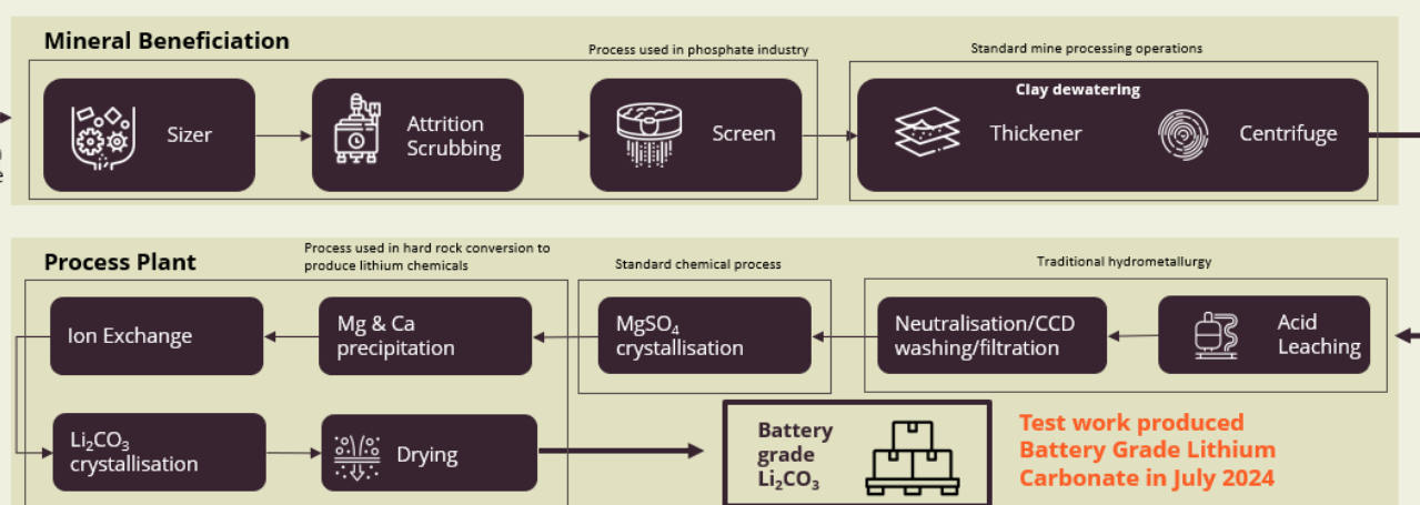
Fig 2 – McDermitt Flowsheet
