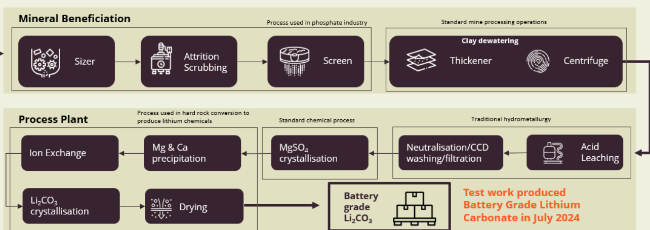
Fig 2 – McDermitt Flowsheet
