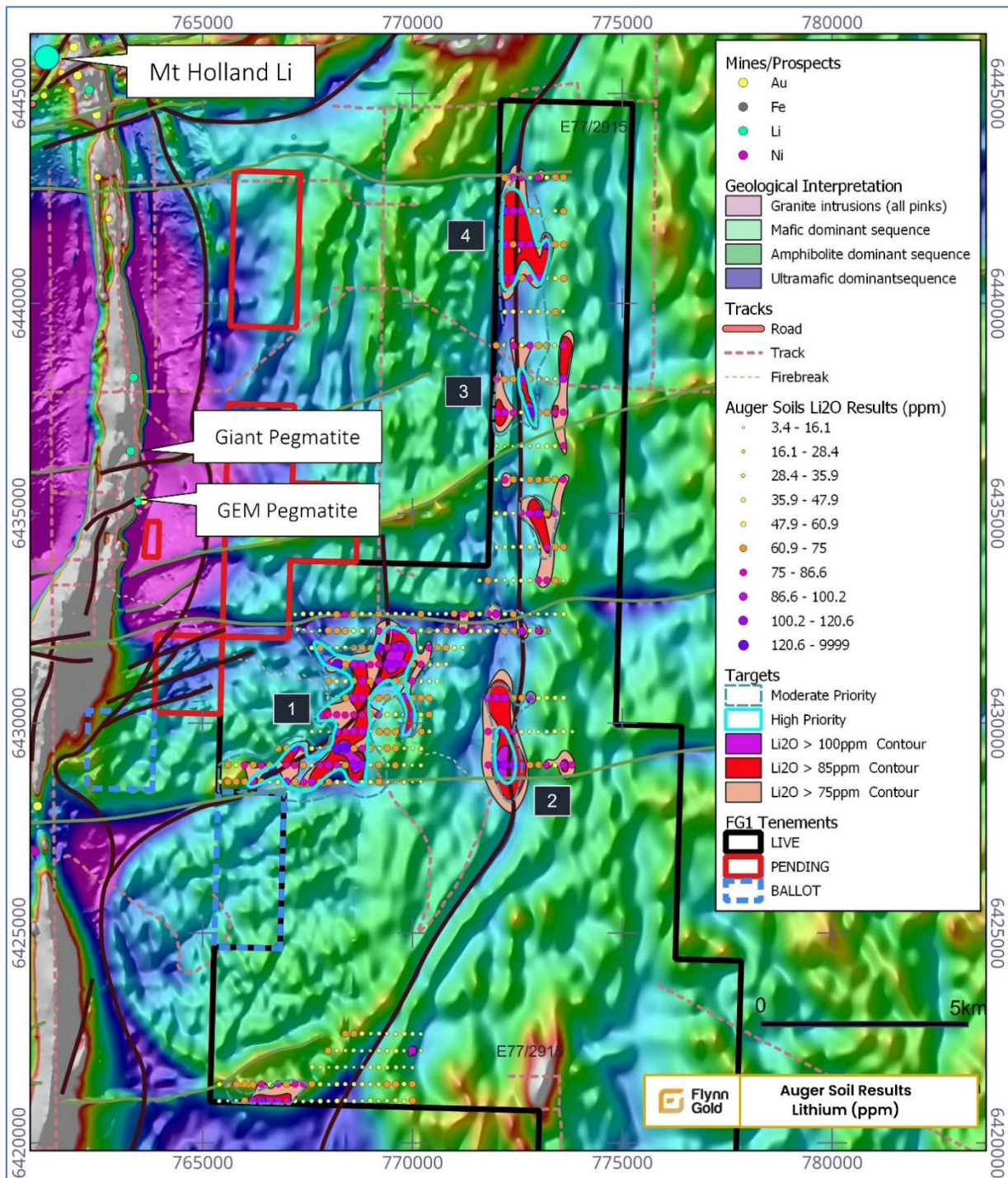
Figure 13 - Auger soil lithium ( \text{Li}_2\text{O} ) results (ppm) over magnetic image showing targets and \text{Li}_2\text{O} contours
