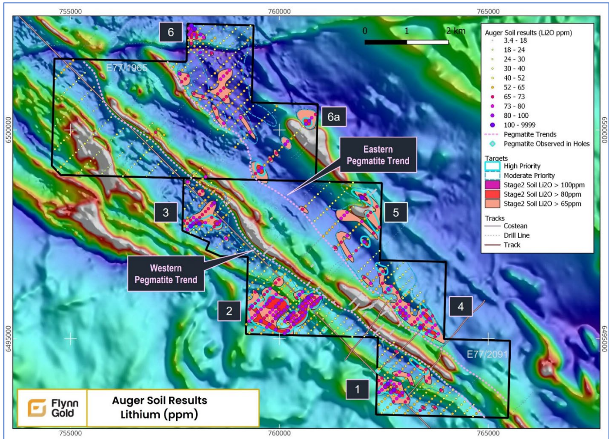
Figure 15 – Auger soil lithium (Li 2 O) results over magnetic image showing targets and Li 2 O contours
