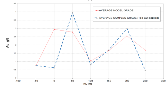
Fig. 3.5-4: Spider-gram constructed for validation of the estimated block model grades, lodes 177 and 178.
