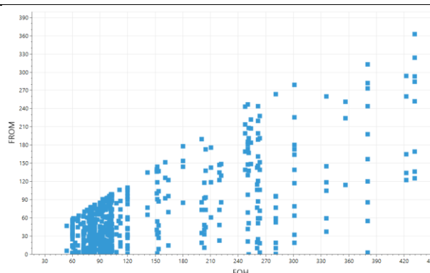
Fig. 2.4-3: Depth of the mineralised intersections vs drillhole length (EOH)
