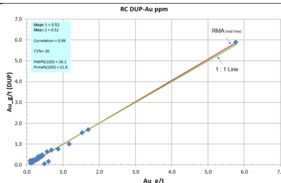
(c) Fig.1.6-1: QAQC diagrams. Blaffo-Guetto prospect exploration drilling, 2021-2022.
