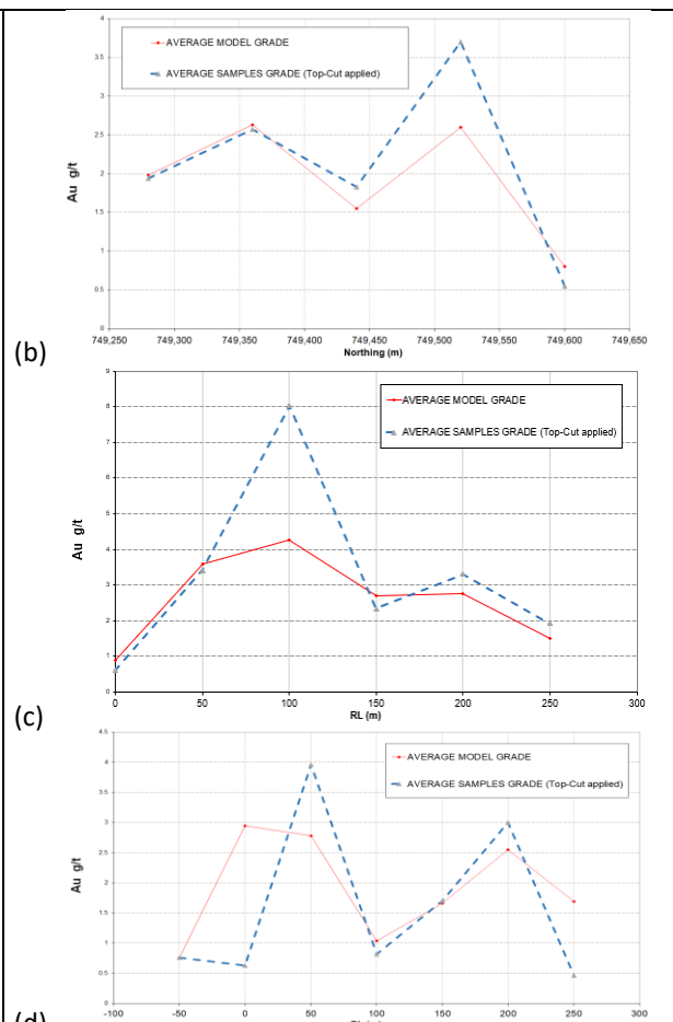
Fig. 3.5-4: Spider-gram constructed for validation of the estimated block model grades, lodes 177 and 178.
