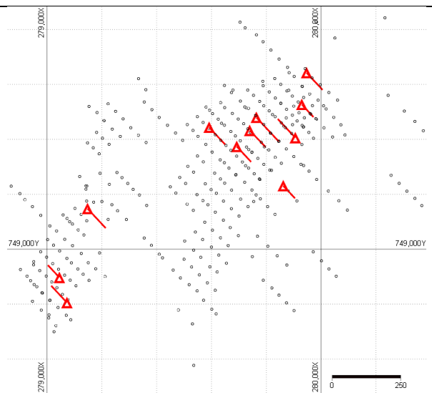
Fig. 2-10-1: Map of the proposed drillholes, denoted by red colour. Collars of the existing drillholes (black dots) are shown for the reference
