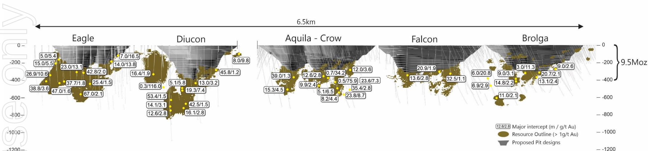
Figure 2: Hemi Schematic Long Section
