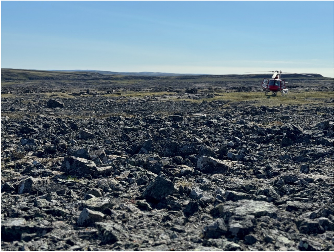
Figure 11 - Typical landscape of the basalt flows at the Kilauea target. Field crew identified native copper alongside chalcocite-malachite-chrysocolla replacing vesicles within the brecciated flow tops for over 120 m strike length.
