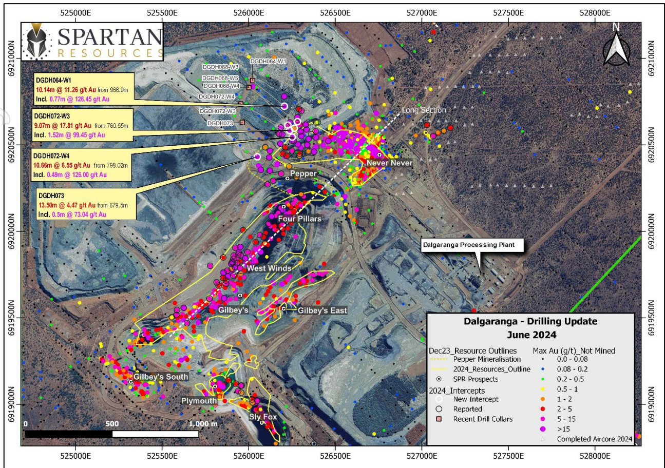
Figure 4: Plan-view of the key gold targets at the Dalgaranga Gold Project. The Pepper Gold Prospect is located between the Never Never Gold Deposit and the Four Pillars Gold Prospect, marking the northern end of the former Gilbey's Open Pit. Drill-hole intercept grades are shown coloured by gold grade and recent drill assays are highlighted in gold callout boxes.
