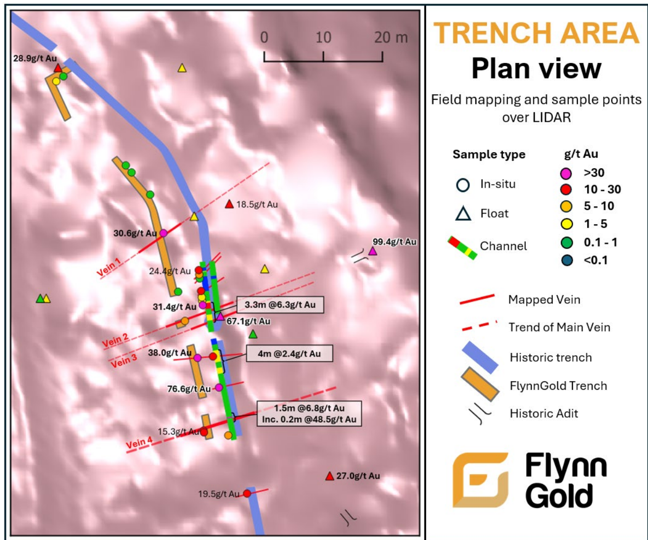
Figure 3 - Plan view of Trench area with sample points and channels
