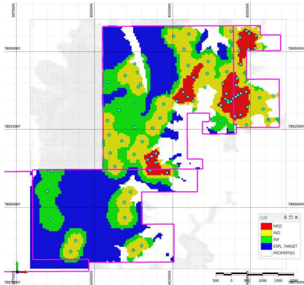
Plan view of the Tiros deposit with the classification of the mineral resources colored by classification.
