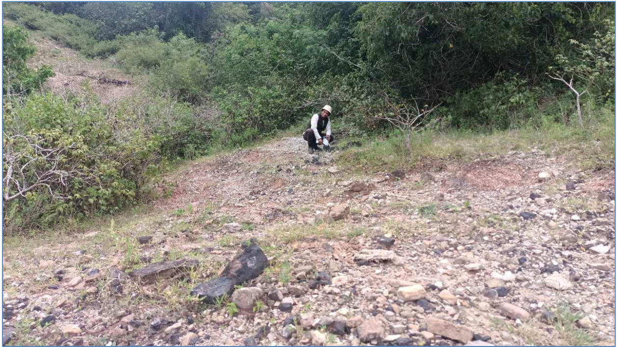
Figure 2: Location of sample CBR114506 showing manganese formation just below the surface in Reconnaissance Permit ESR-RP-01, 7km along strike from the Lalena Prospect; greater than 80% of the sample was logged as manganese and iron oxides.
