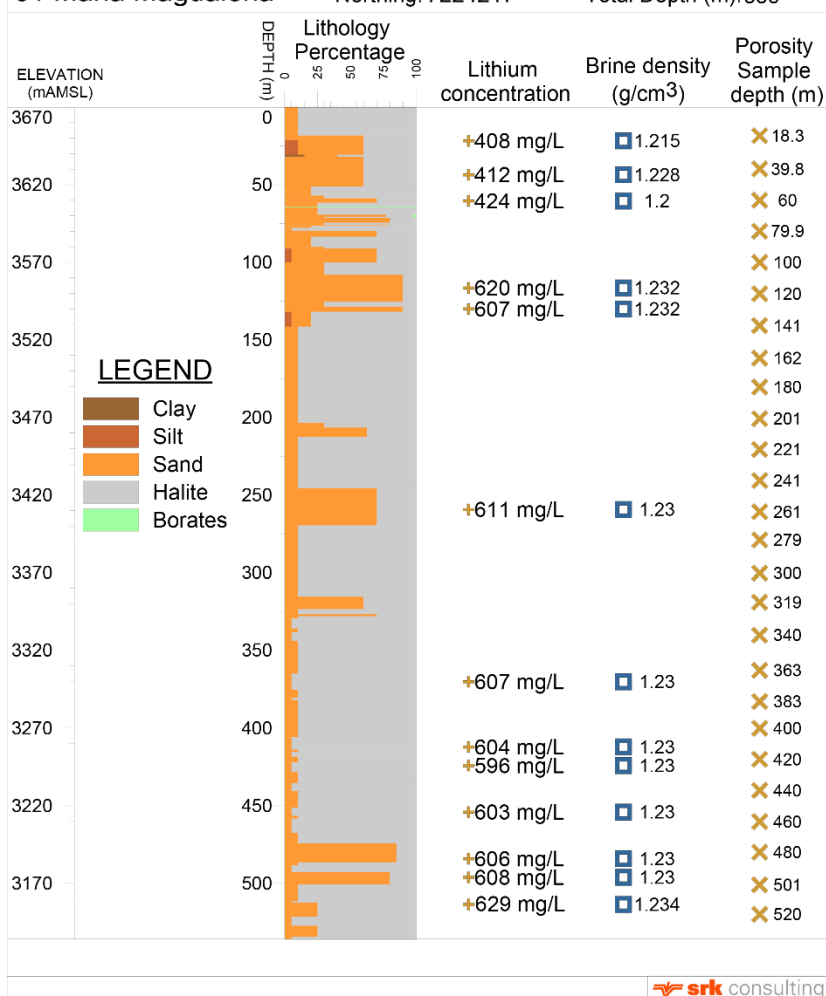
Figure 1 – Lithological section showing the continued presence of good quality, porous and permeable sands and high-grade Lithium concentrations
