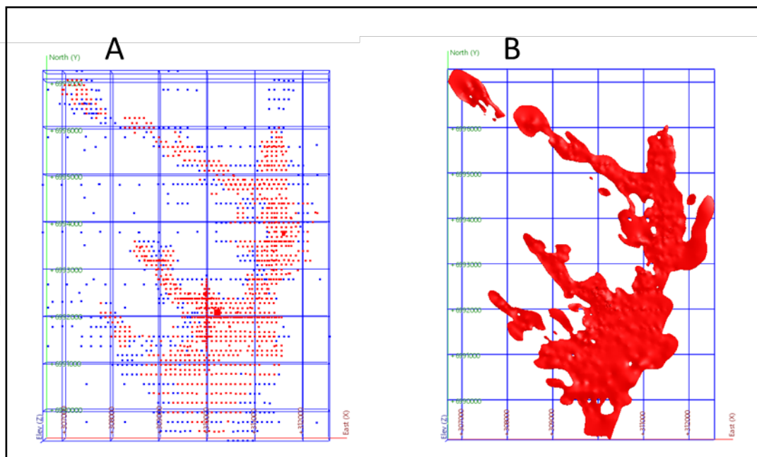
Figure 7: (A) Indicator data, in red all holes with a maximum 0.5m composite value over 1b00ppm (included) and in blue all holes without a maximum 0.5m composite value of 100ppm (discarded). (B) Final Lake Maitland 100 ppm mineralisation envelope in plan view.
