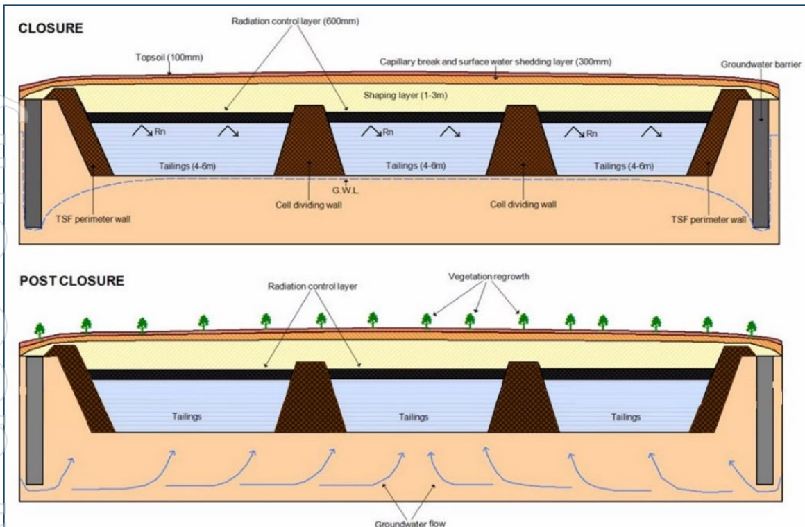
Figure 24: Schematic of the TSF at closure (top) and post-closure (bottom).
