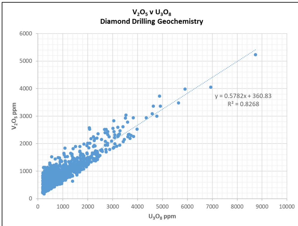
Figure 9: Bivariate plot showing the relationship between U 3 O 8 and V 2 O 5 (calculated from U and V respectively) in the geochemistry from all diamond holes inside the 200ppm U 3 O 8 cut-off within the Lake Maitland U 3 O 8 resource.
