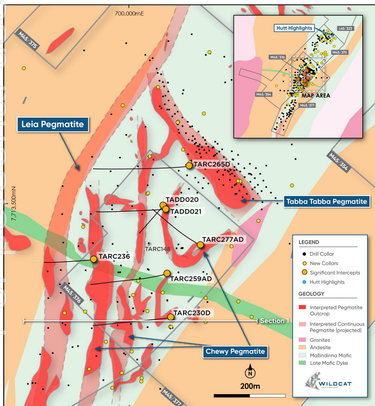
Figure 2 – Plan view of drilling (previously reported: black, new: yellow) at Leia since ASX Announcement dated 10 April 2024. Drill collars with significant intercepts appearing in the highlights are displayed in orange. Section line relates to Figure 4.
