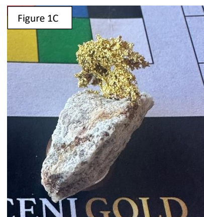
Figure 1 Gold* bearing quartz specimen vein sample collected from the sample trench over the Christmas Gift shear.
