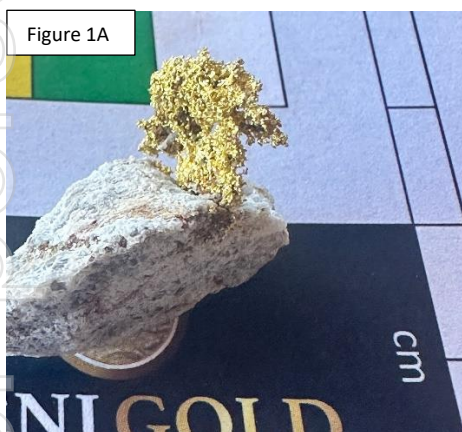
Figure 1 Gold* bearing quartz specimen vein sample collected from the sample trench over the Christmas Gift shear.
