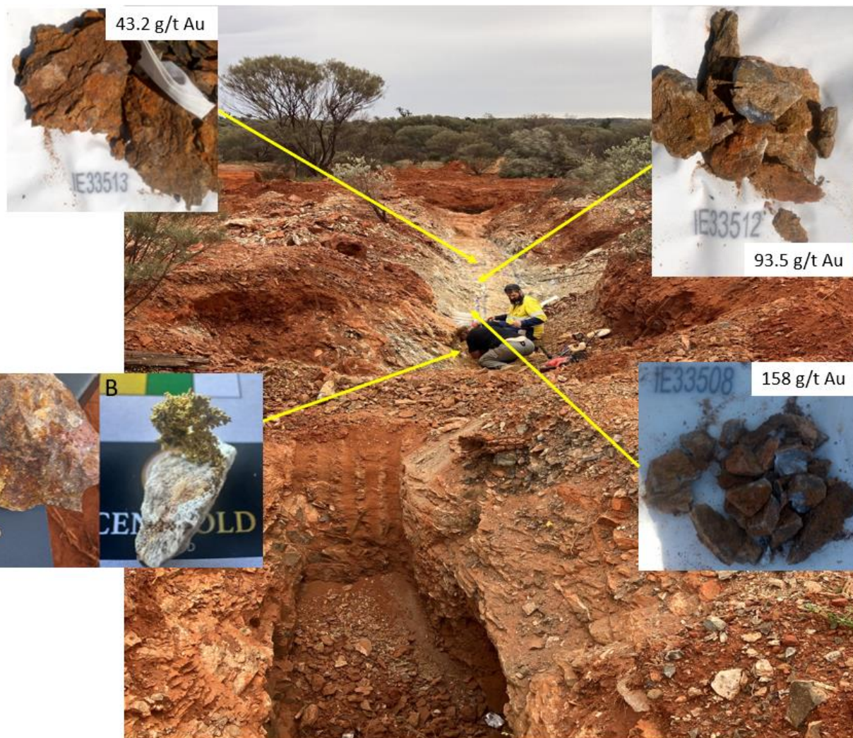
Figure 3: Photo of exposed geology within the recently expanded sample pit looking north (310 degrees) with historic shaft in foreground. IcenI Gold senior geologist and prospector inspecting and collecting gold bearing quartz stringers. Approximate location of significant rock chip sample results and recently collected gold bearing quartz veinlets shown.
