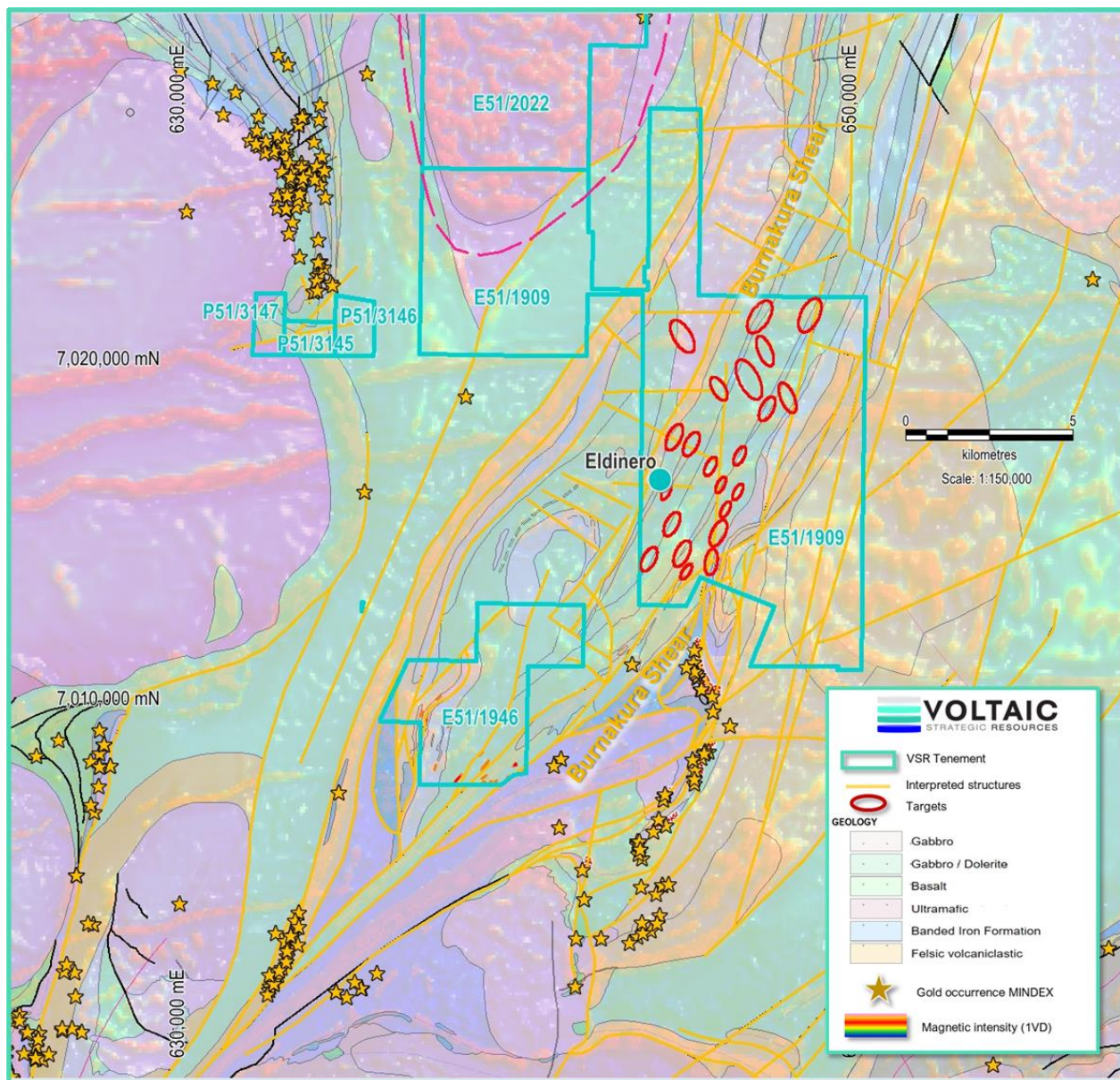
Figure 4. Regional geology overlay on airborne magnetic image.
