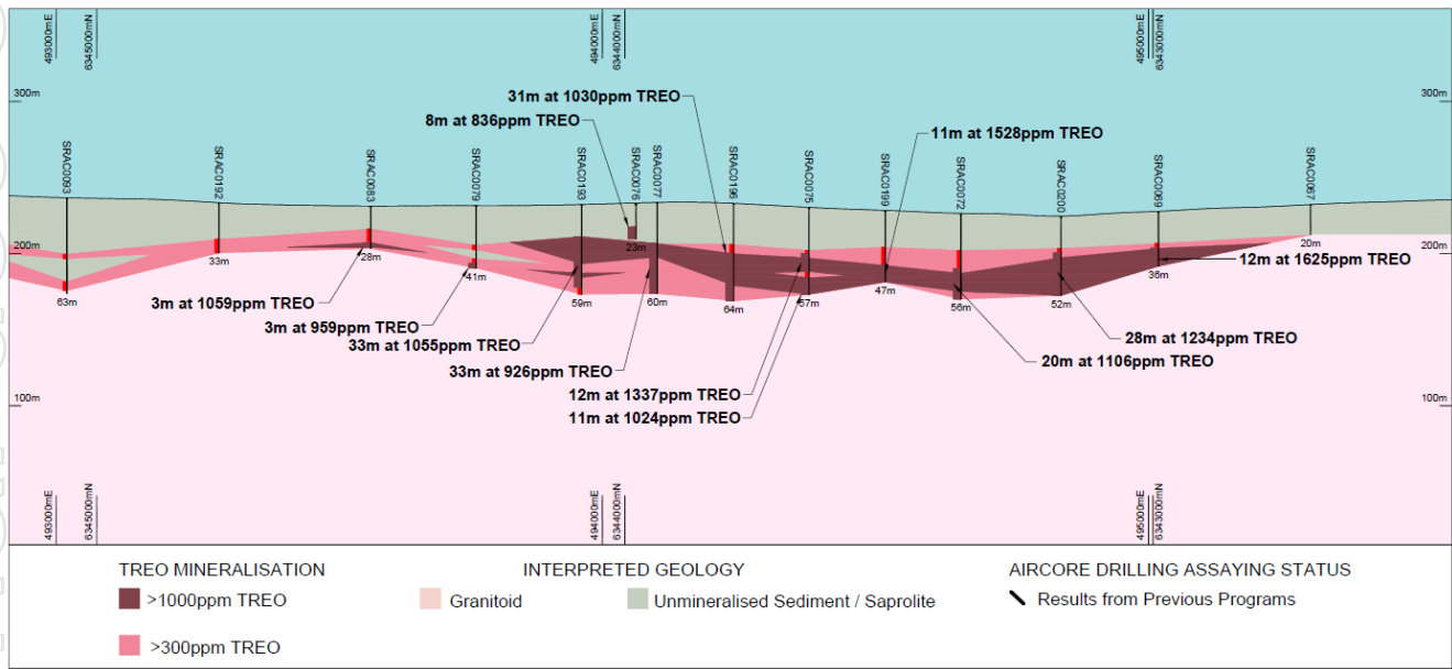
Figure 9: Scrum Prospect Cross Section F to F' (refer Figure 19 for cross-section location). Vertical exaggeration x 5. (Source: OD6)
