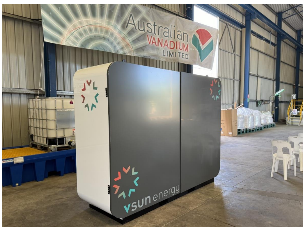
Figure 1 – Residential VFB prototype pictured at the vanadium electrolyte manufacturing facility
