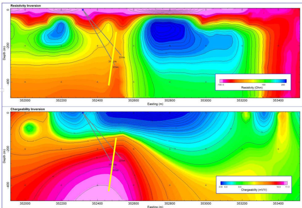
Figure 3. Dipole-Dipole IP pseudo-section just north of tenement boundary and showing Miramar diamond drill hole traces (approximately 40m off-section to the north).
