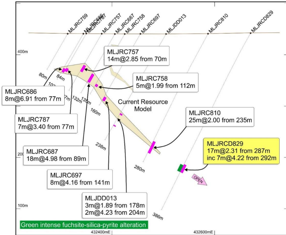
Figure 5. Cross section for LN4 northern area showing high-grade dipping gold zone containing resource model outline and MLRCD829 being a down dip extension of over 75m with intense fuchsite alteration.
