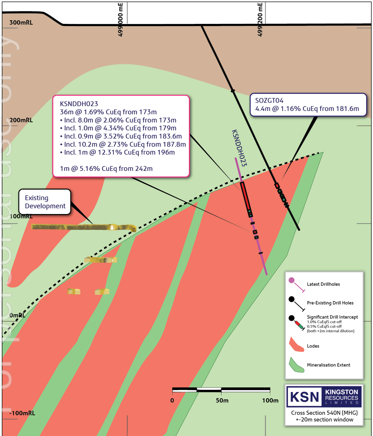
Figure 4: Cross section of drill hole KSNDDH023.
