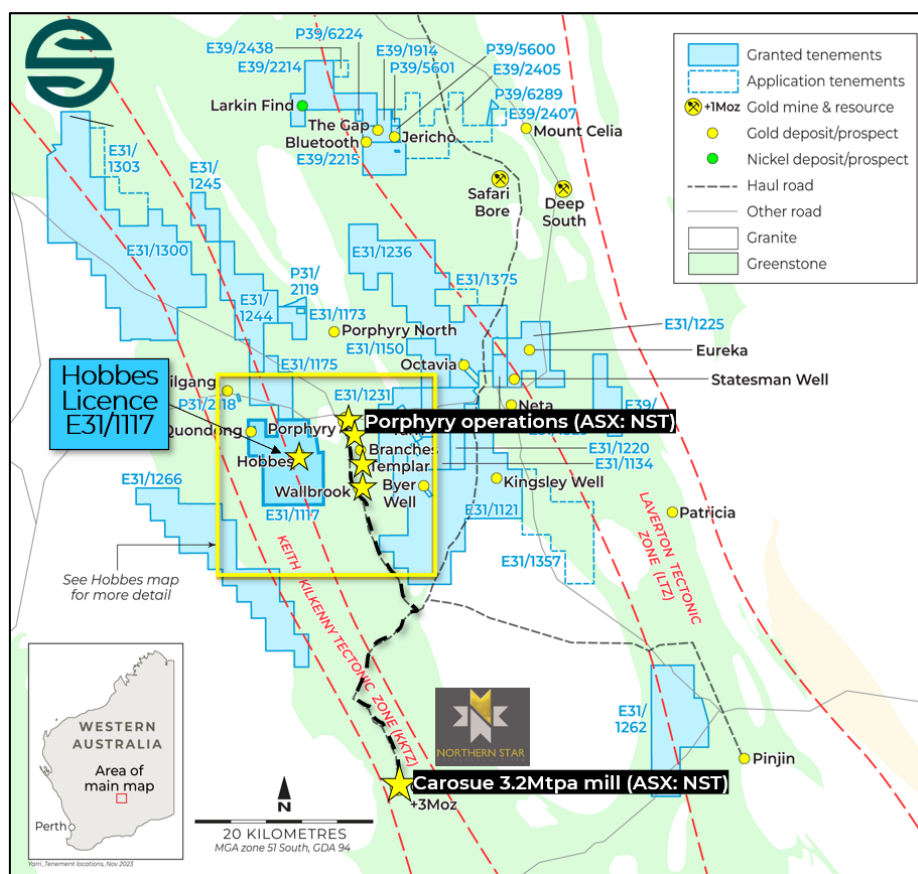
Figure 1. Location of the Hobbes Licence within the Company's 1500km 2 Yarri Project tenure.
