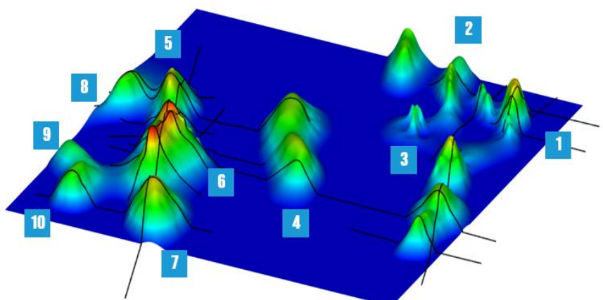
Figure 8: Lead inventory showing proposed 2D seismic program (structural leads derived from airborne gravity data)
