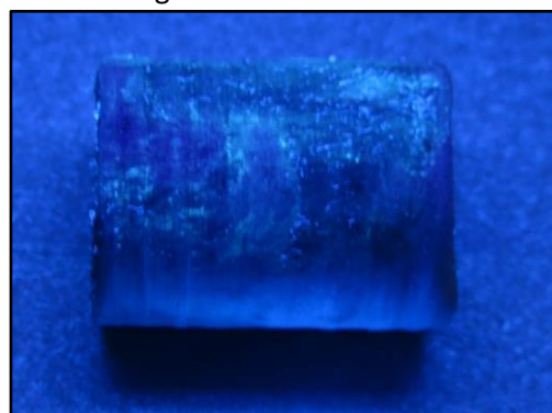
Figure 1: SWC sample retrieved from Hickory-1 showing fluorescence
