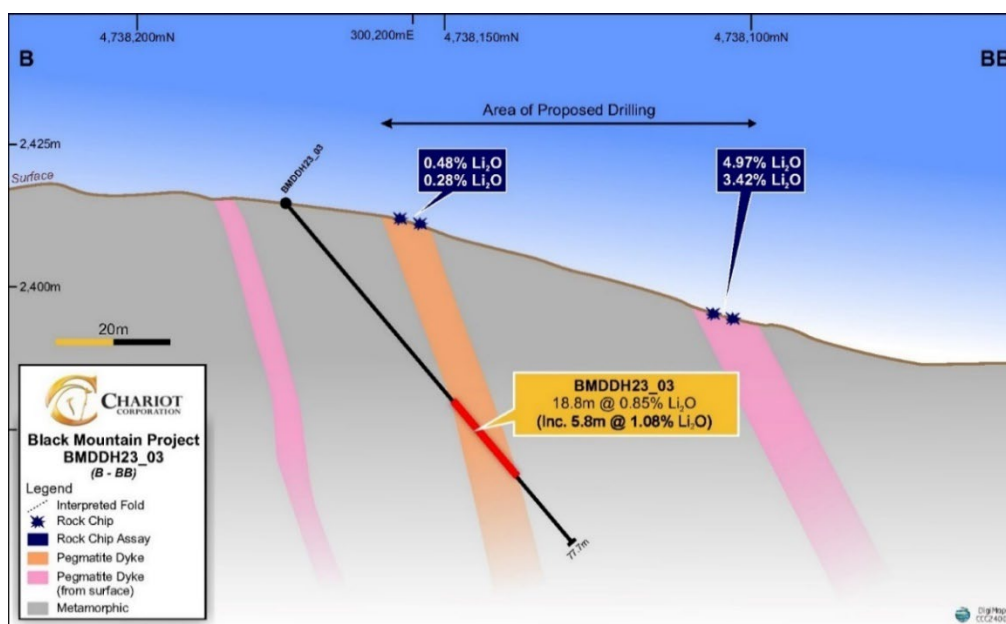
Figure 3 Cross section showing BMDDH23_03 drill trace with the intersected pegmatite shown in red.
