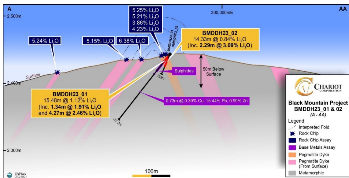
Figure 2 Cross section showing BMDDH23_01 and BMDDH23_02 drill traces with the intersected pegmatite shown in red.
