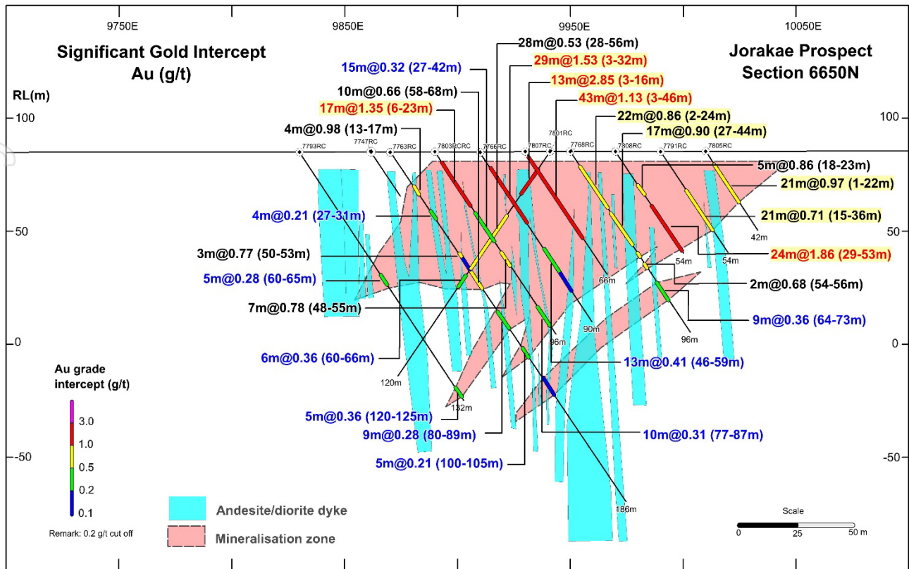
Figure 3: Cross section 6650N showing significant Au intercepts, Jorakae prospect
