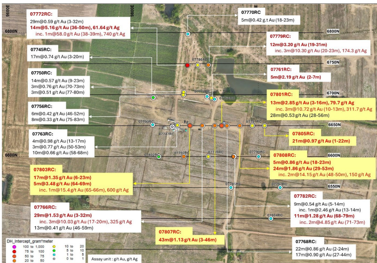
Figure 2: Significant Au intercepts in RC, Jorakae prospect
