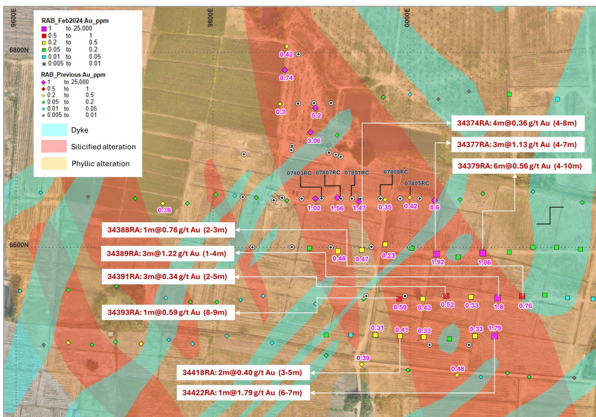
Figure 1: Significant Au intercepts in RAB, Jorakae prospect
