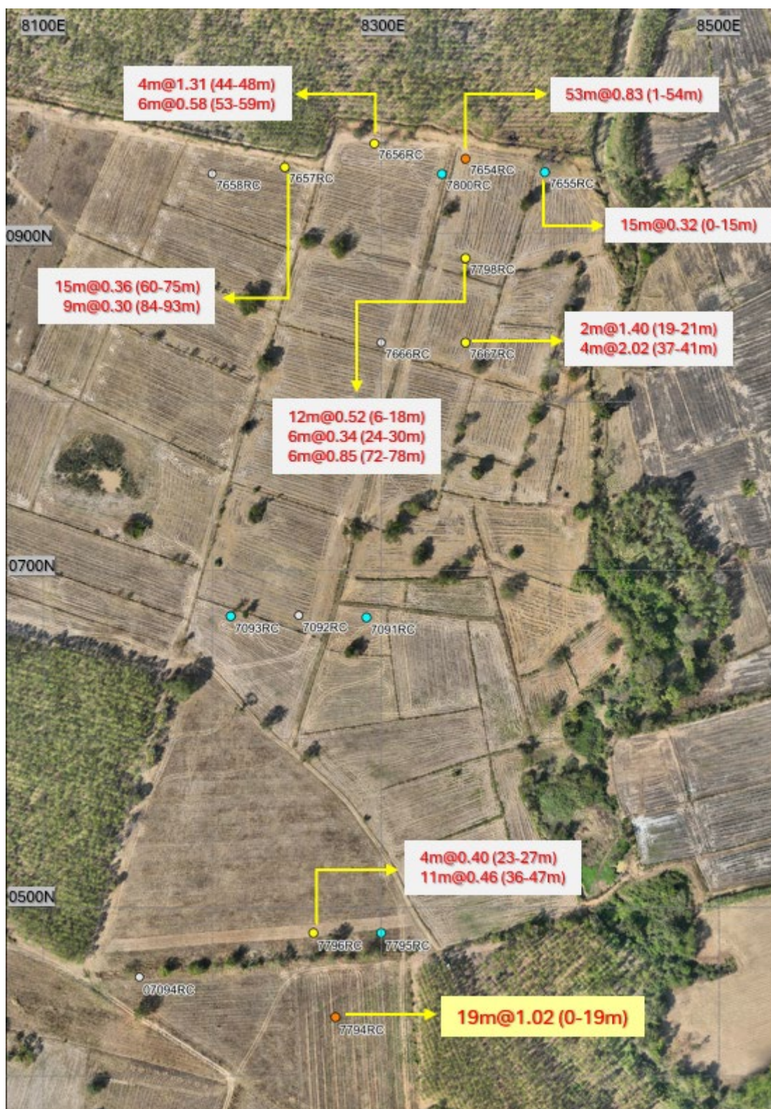
Figure 4: Significant Au intercepts in RC, Chalawan prospect
