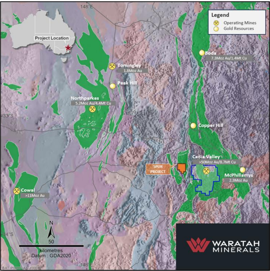
Figure 1: Spur Project location (total metal endowment – refer references: Phillips 2017, Newcrest 2023, CMO 2023, Evolution 2023, Alkane 2023, Regis 2023)
