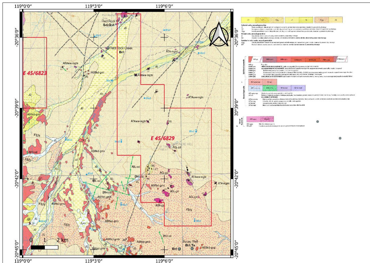
Figure 13: Surface geology of EL applications E45/6823 and E45/6829. (after GSWA 1:100k Carlingdie 2756 geology sheet)
