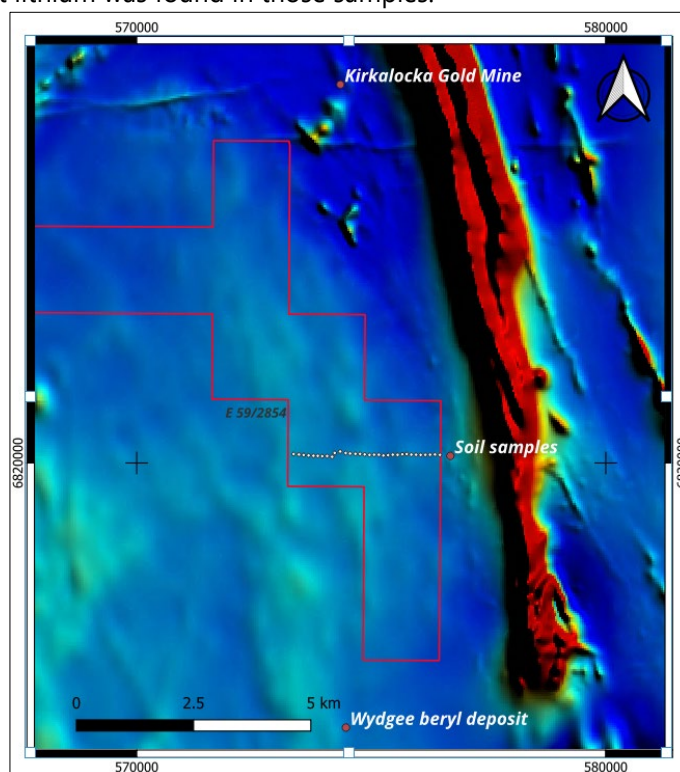
Figure 10: Soil sample locations E59/2854. (after GSWA aeromagnetics 40m RTP 2023)
