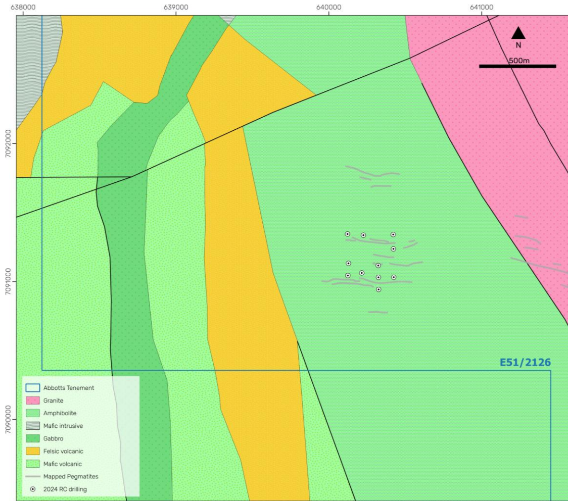
Figure 1: Geological map of the Buttamah Prospect with collar locations of completed RC drilling.
