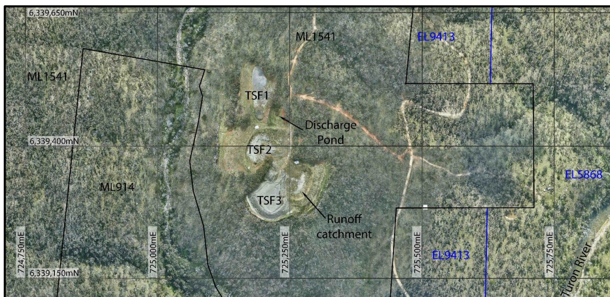
Figure 20 – Current arrangement of tail storage facility
