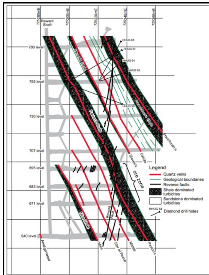
Figure 9 - Cross section at 6,341,555mN through the Reward shaft
