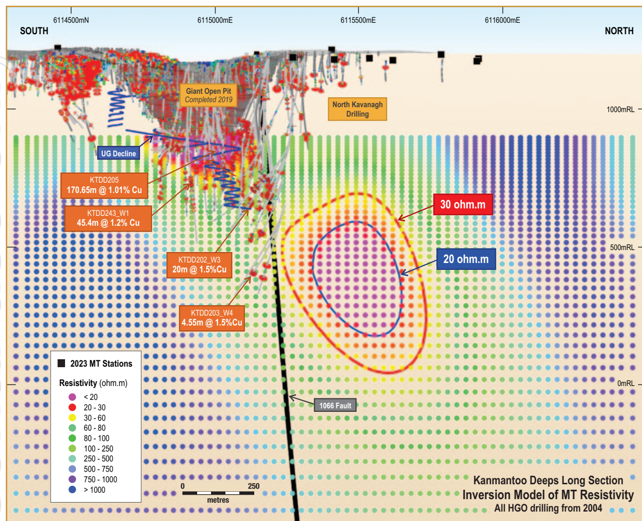
Figure 3: Kamantoo Deeps Long Section.
