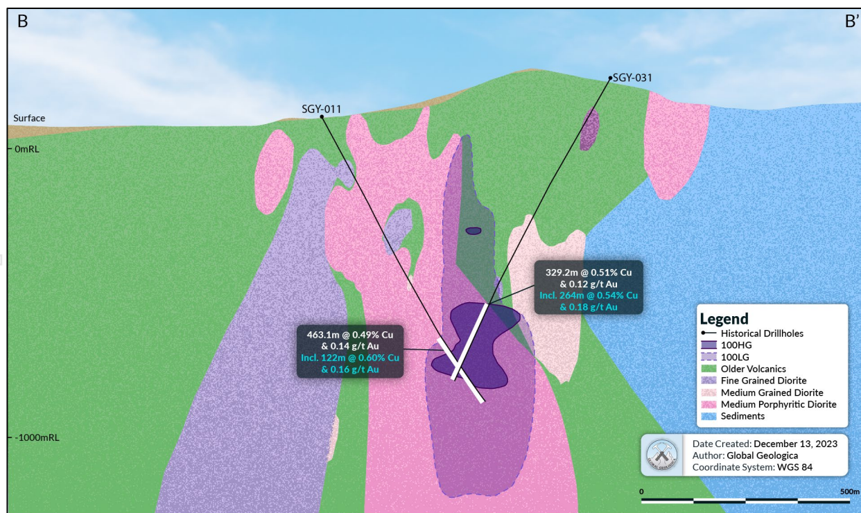
Figure 6. Oblique Cross Section B-B' showing the location of the 100LG and 100HG mineralised domains.
