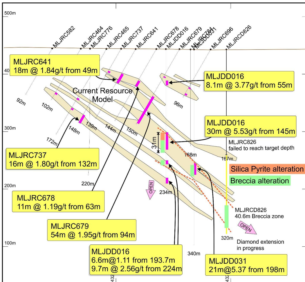
Figure 2. Cross section for LJA4 centre area showing thickened high-grade dipping gold zone containing breccia and silica-pyrite alteration, resource model outline, thickened mineralisation in drill hole MLJRC679, breccia zone in MLJDD016 and MLJDD031 and depth extensions downdip with a thick 40.6m thick breccia in MLJRCD826, which is still open to the east with assays pending.
