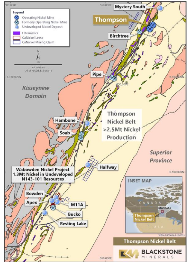
Figure 2: Thompson Nickel Belt in Manitoba, Canada
