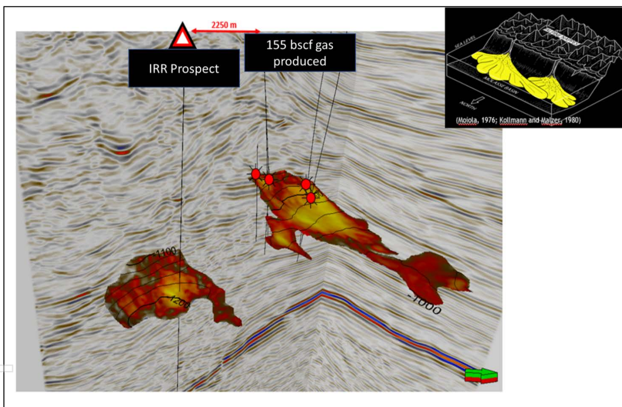
Figure 2: 3D rendering of the IRR prospect mapped on 3D seismic and supported by AVO anomalies indicating gas filled reservoir. IRR is an analogy to the close by gas field. The insert shows the geological model suggesting the reservoir stemming from turbidite deep water sediments
