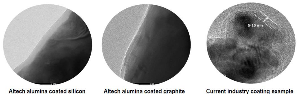
Altech alumina coated silicon Altech alumina coated graphite Current industry coating example
